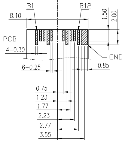
RECOMMEND PCB LAYOUT BOTTOM VIEW
